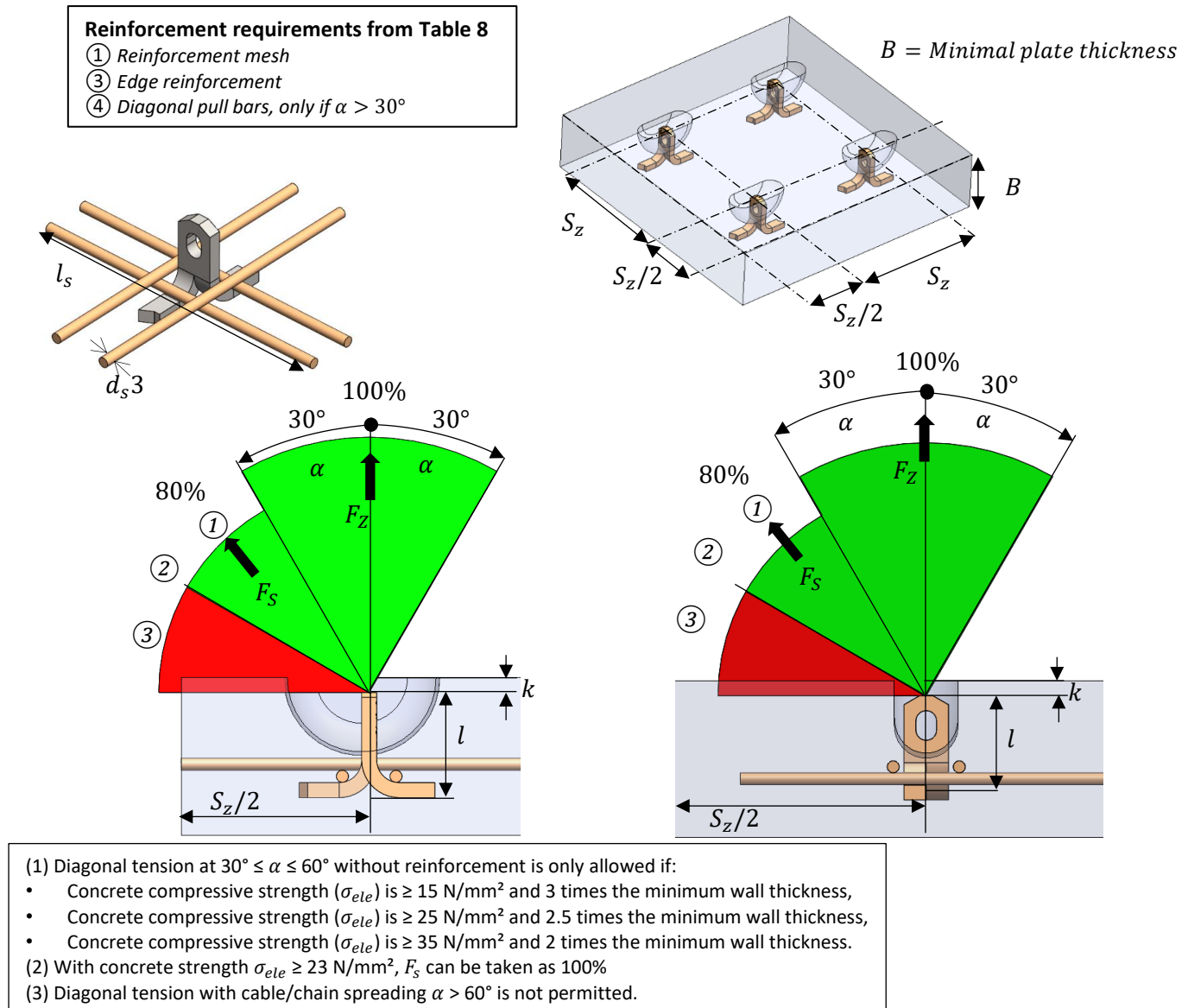
Figure 10 Reinforcement requirements for STA F anchors.
