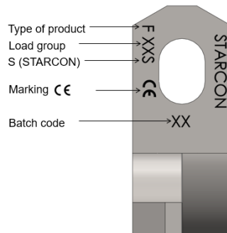
Figure 2 Marking on top of the STA F.
